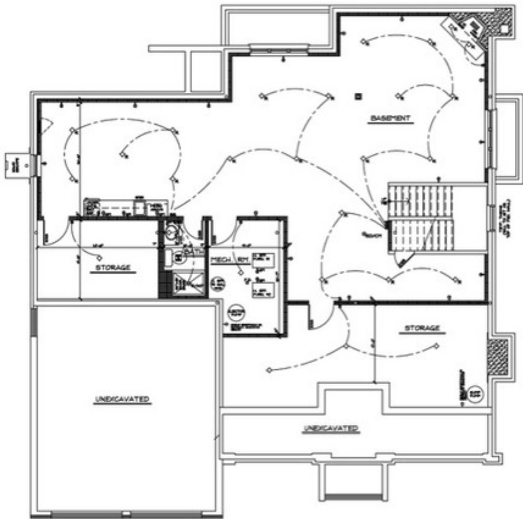
FINISHED BASEMENT PLAN
