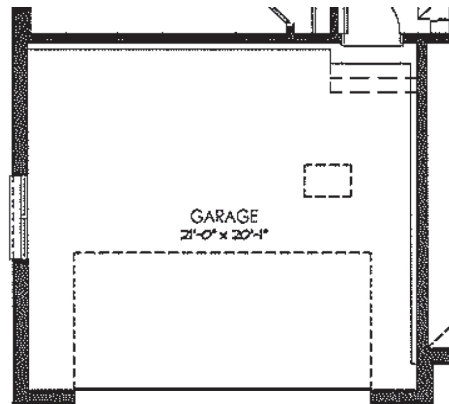
OPTIONAL FRONT LOAD GARAGE PLAN
