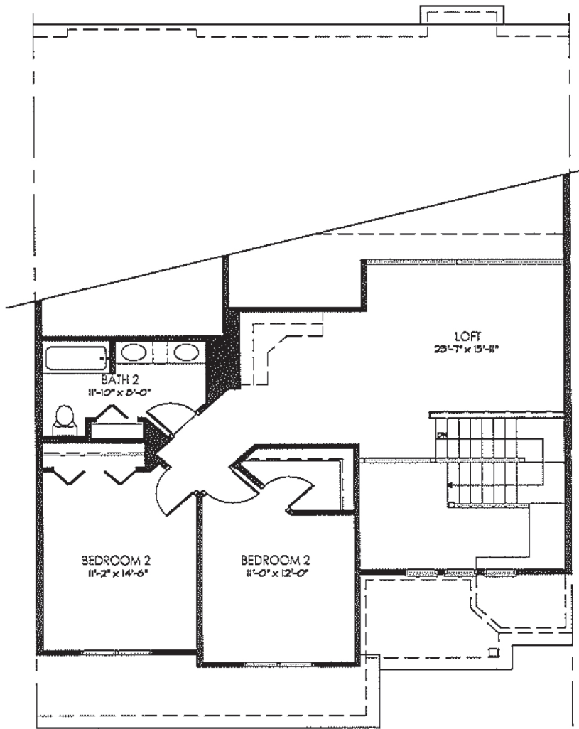
UNIT C SECOND FLOOR PLAN
